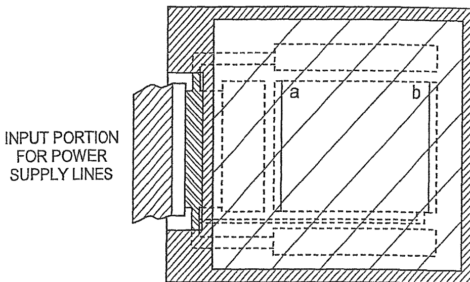
FIG. 24 PRIOR ART
