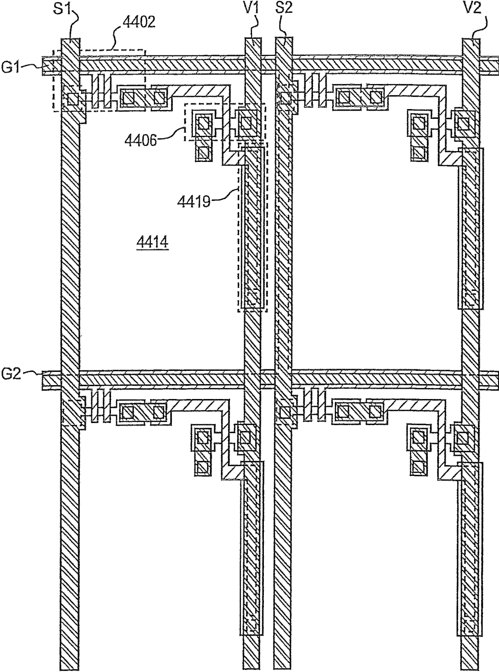
FIG. 41 PRIOR ART
